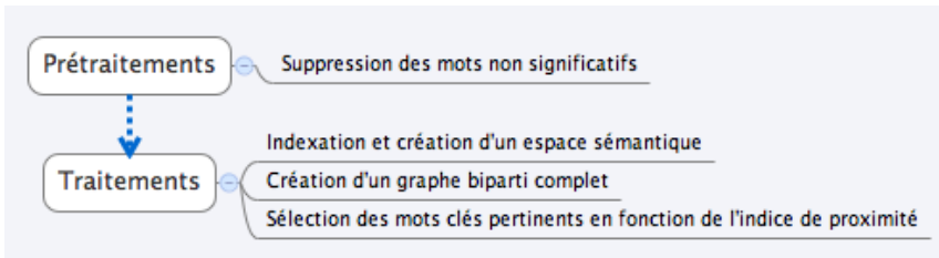
FIGURE 3 – Notre algorithme.
