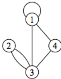
FIGURE 1 – Multigraphe.
